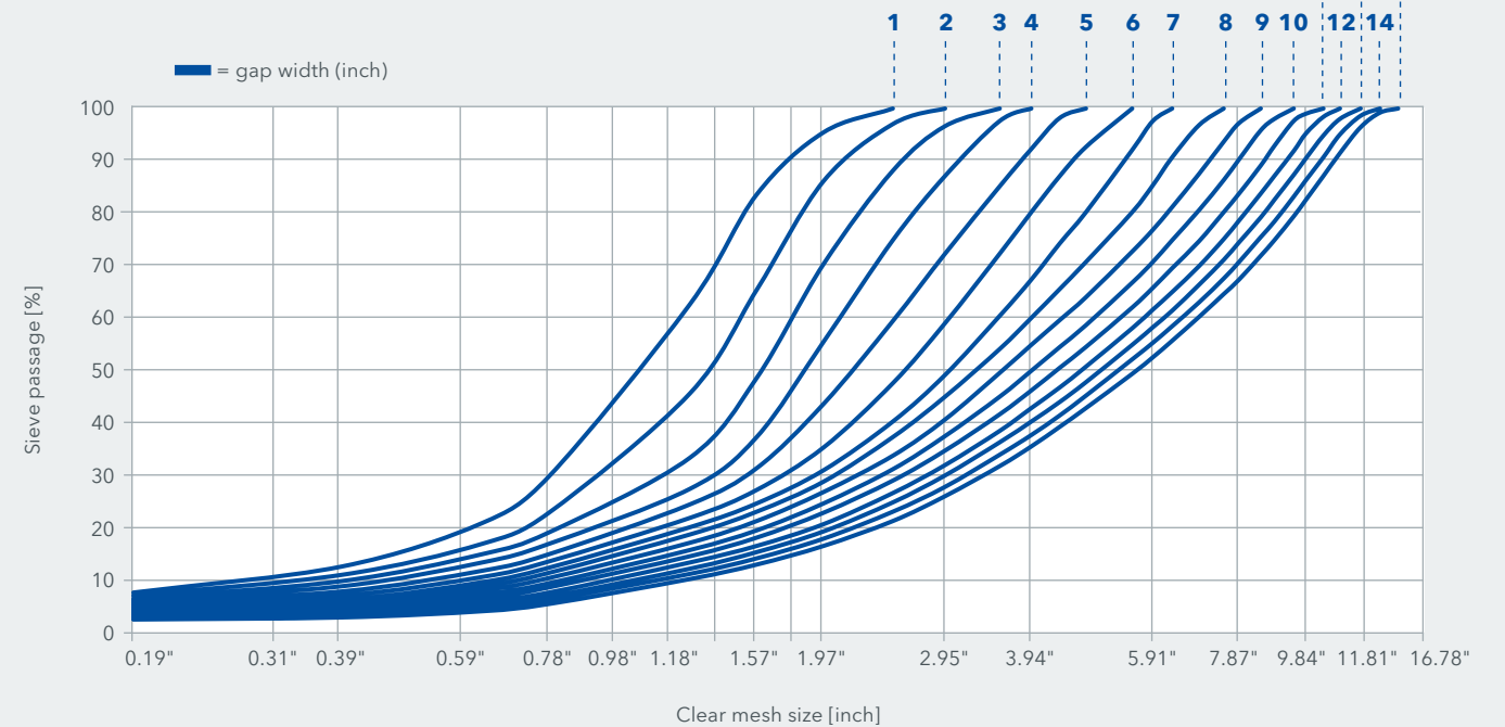
MOBICAT MC 110i EVO2 crushing curve
